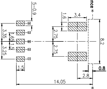
Recommended PCB Layout Tolerance: ±0.1 (Top view)
